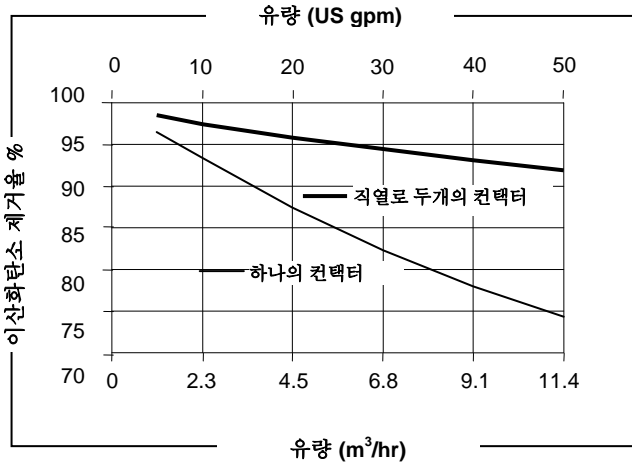
시험조건: X50, Air Sweep Mode, G/L = 3, 20 °C
