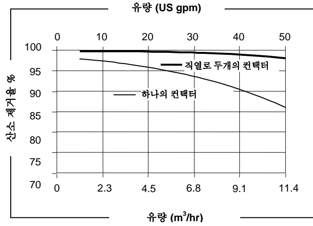
시험조건: X40, G/L 2%, Combo Mode, N 2 스위프, Vacuum Sweep 75 torr, 20 °C
